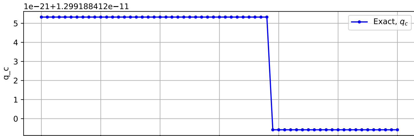
Trajectory No. 1184
