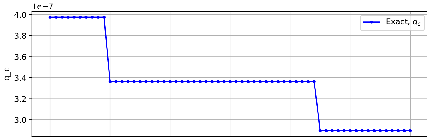
Trajectory No. 1234
