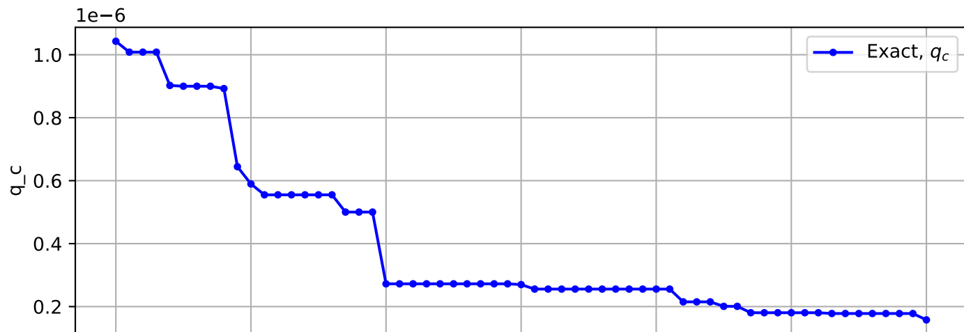
Trajectory No. 1314
