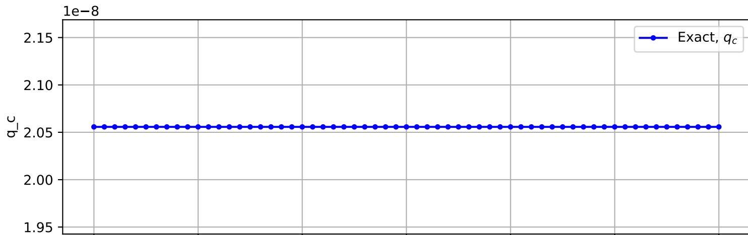
Trajectory No. 1346
