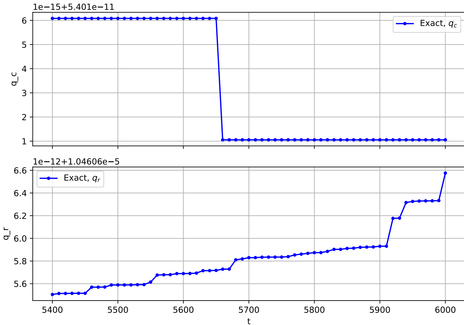
Trajectory No. 1394
