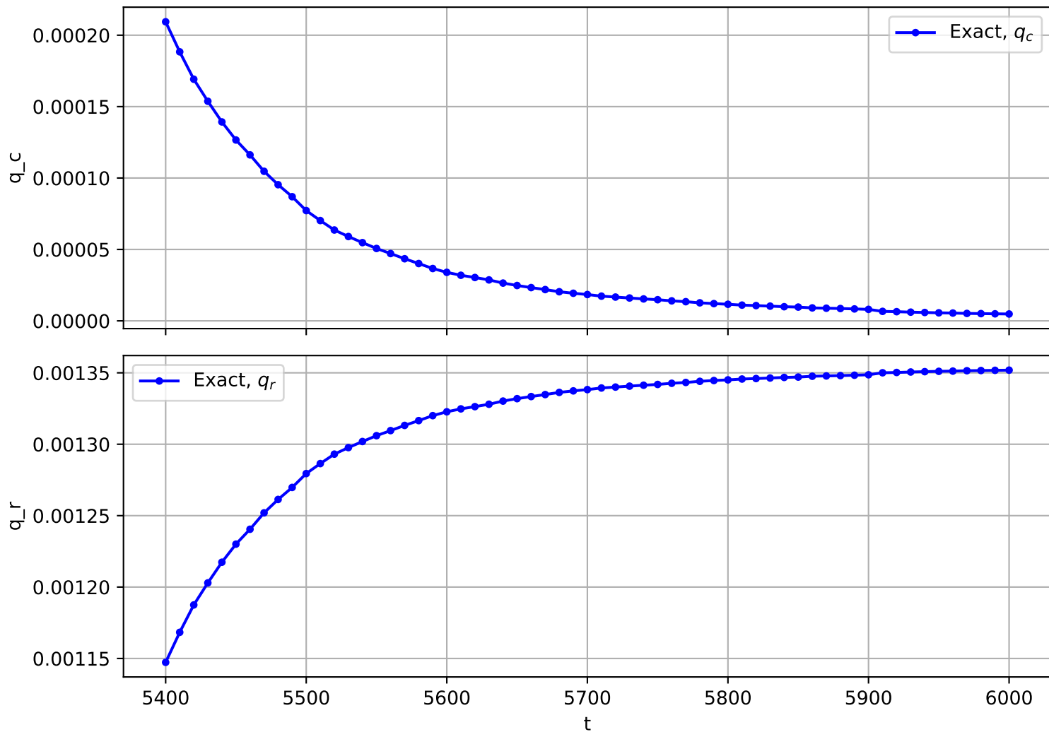
Trajectory No. 1569
