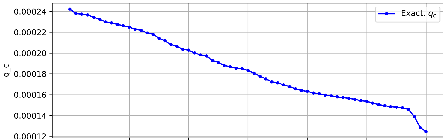
Trajectory No. 1576
