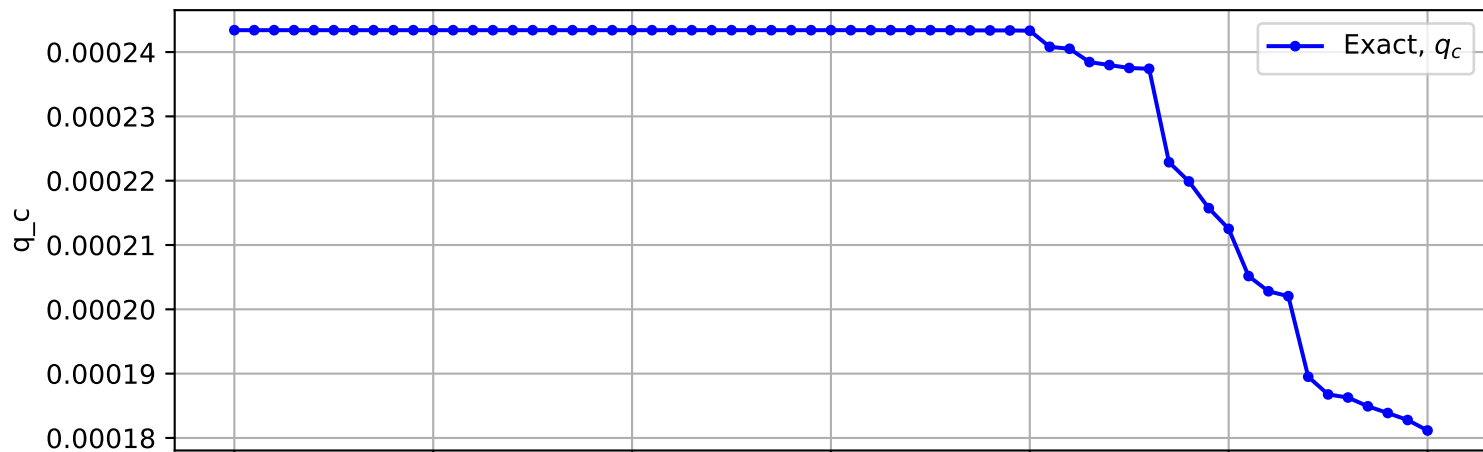
Trajectory No. 1596
