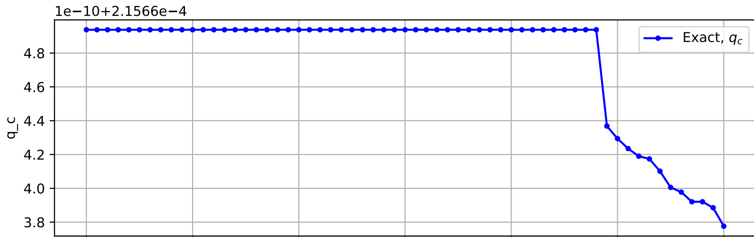
Trajectory No. 1600
