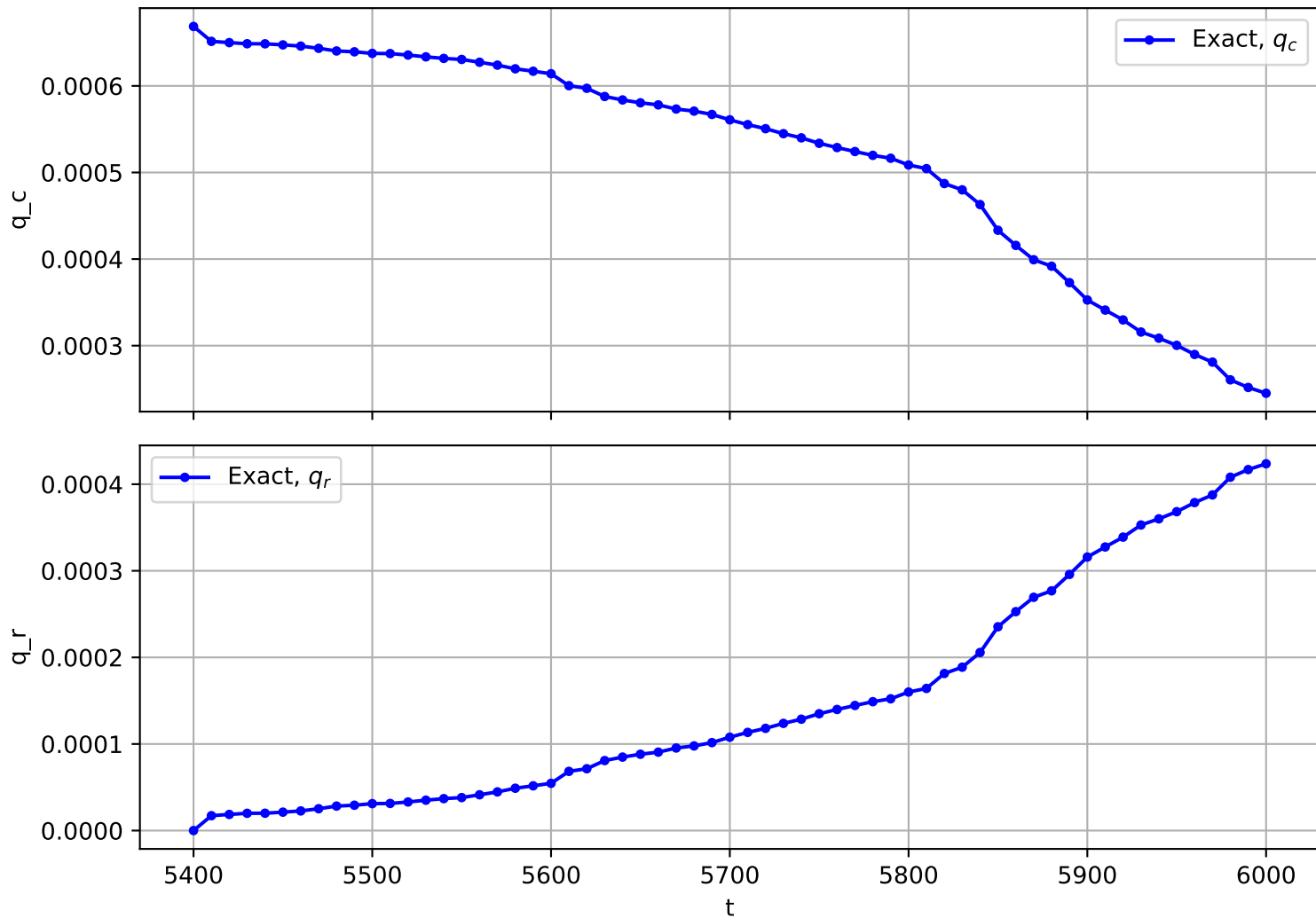
Trajectory No. 1610
