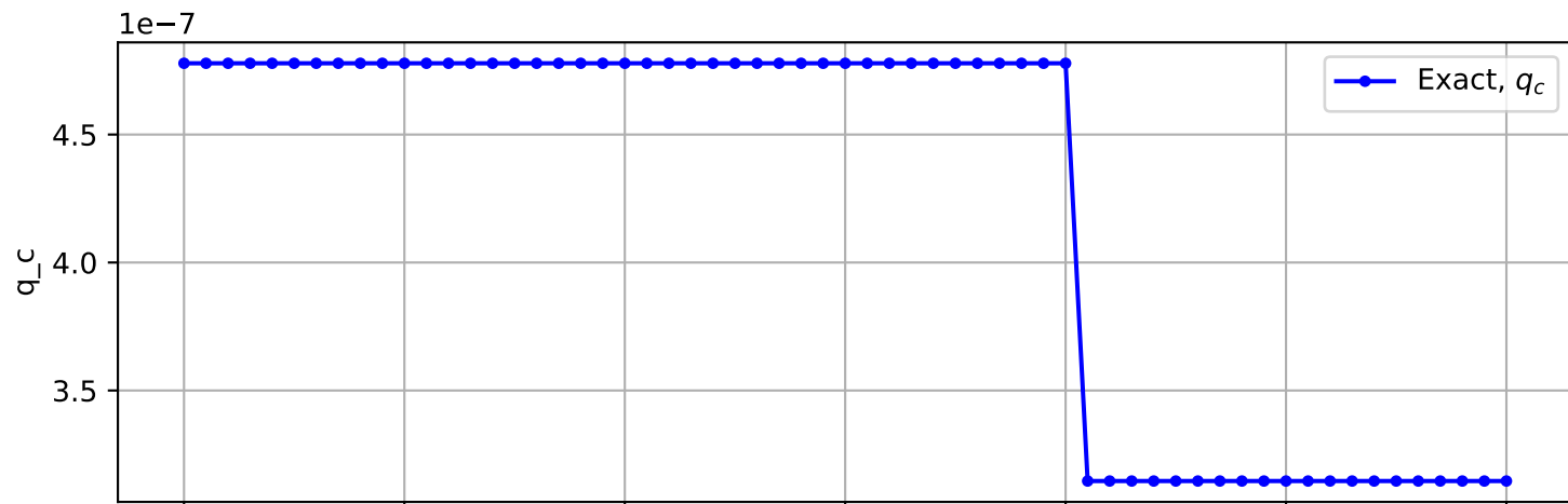
Trajectory No. 1612
