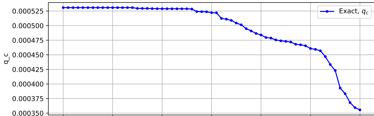
Trajectory No. 1625
