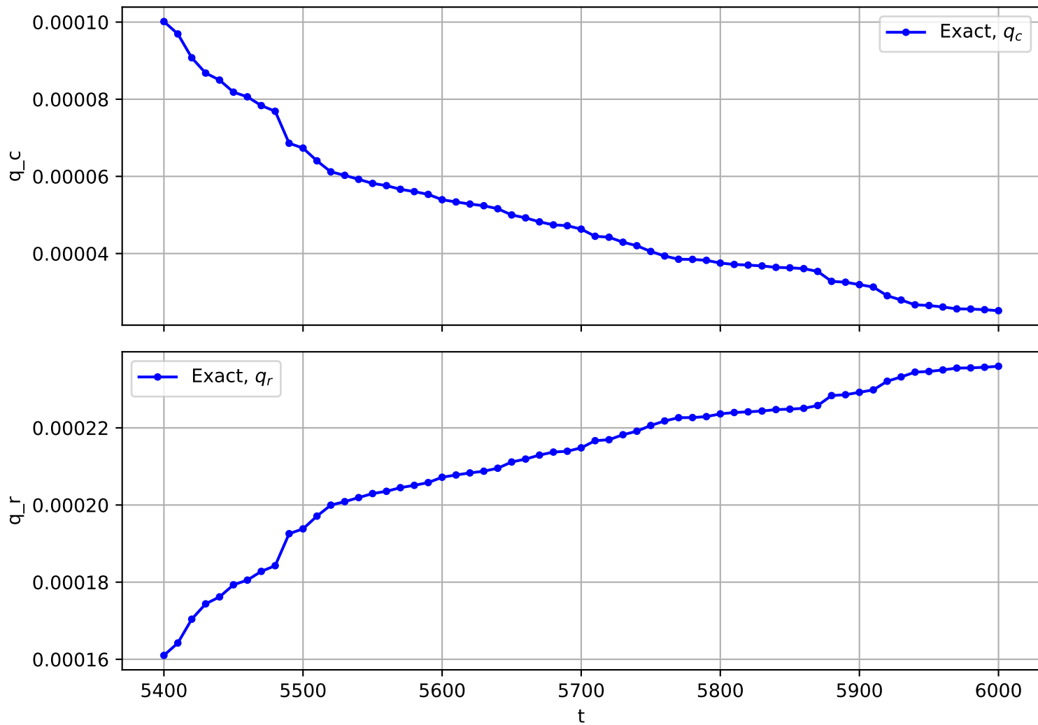
Trajectory No. 1676
