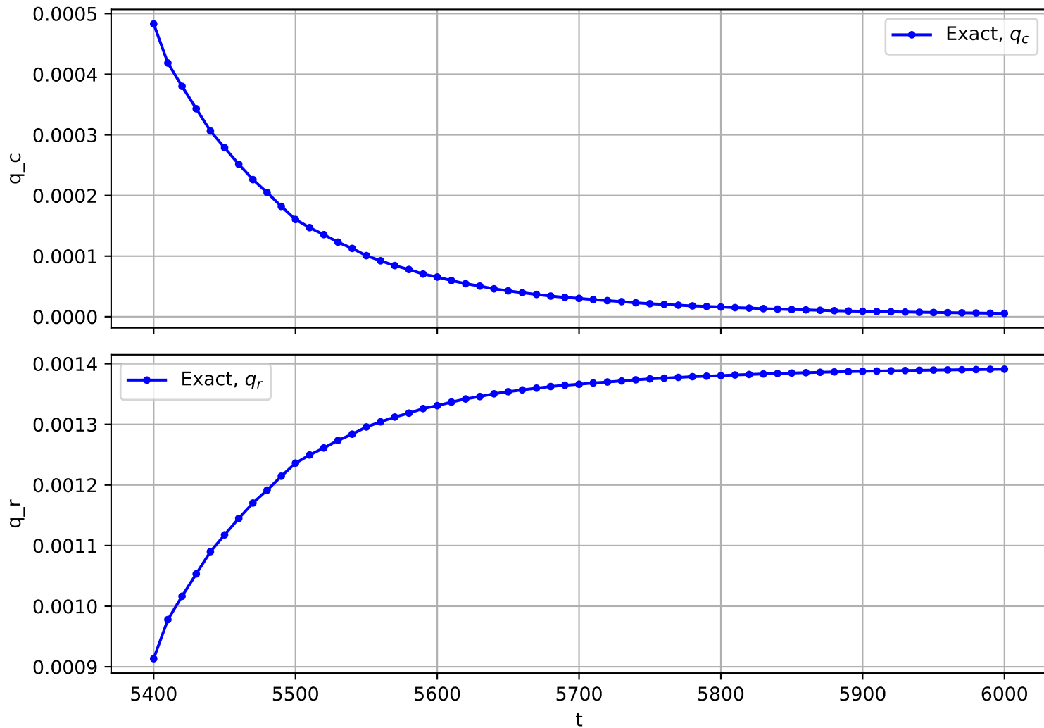
Trajectory No. 1686
