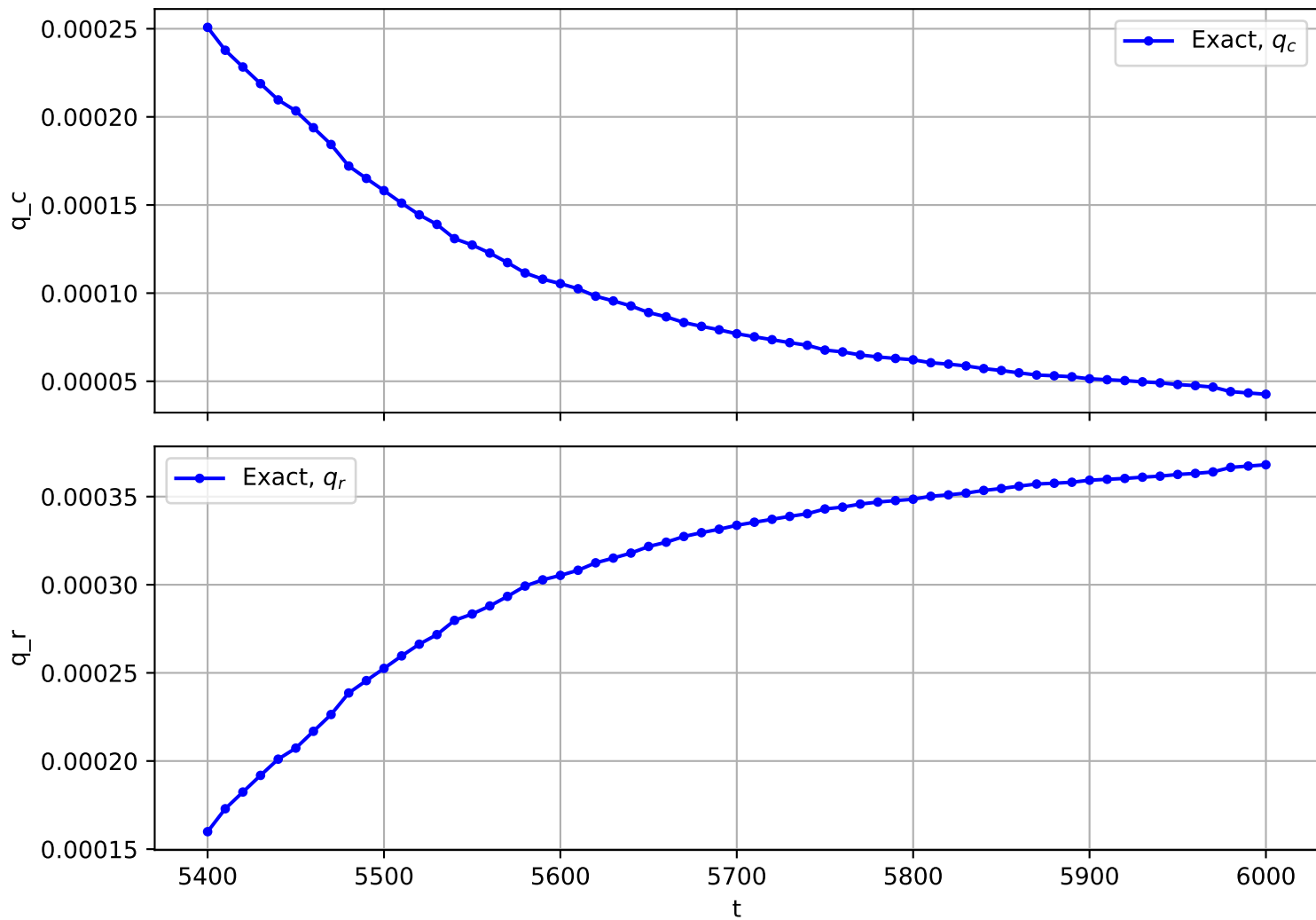
Trajectory No. 1709
