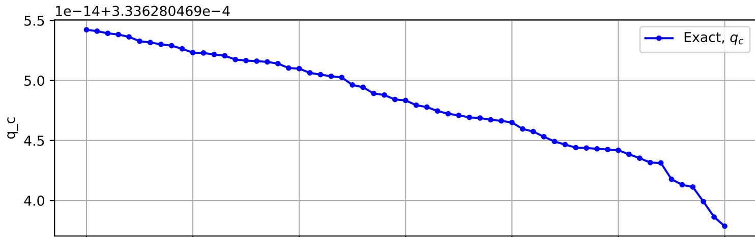
Trajectory No. 1737
