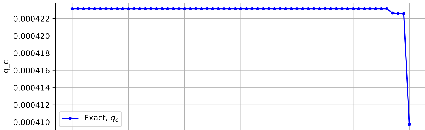
Trajectory No. 1742
