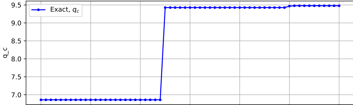
Trajectory No. 1765
