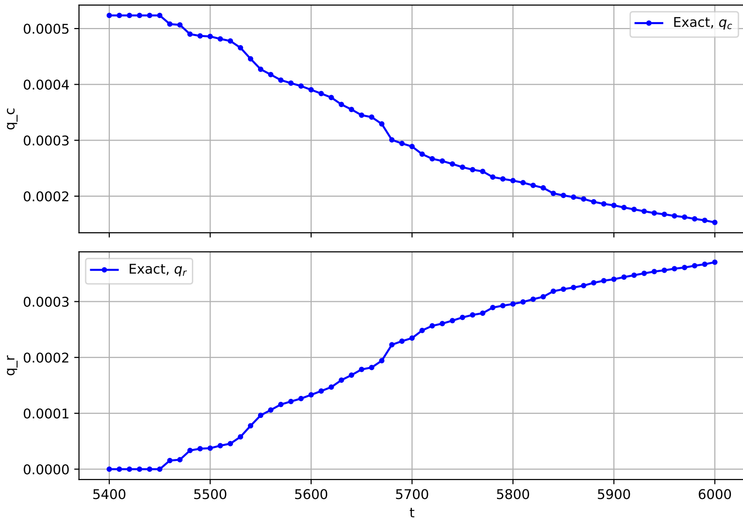
Trajectory No. 1774
