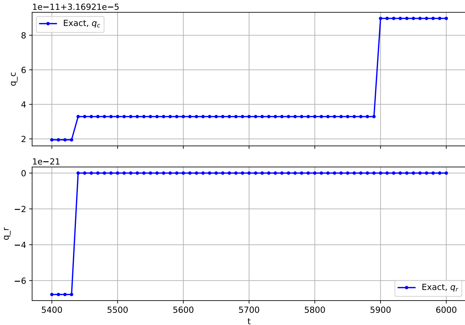
Trajectory No. 1781
