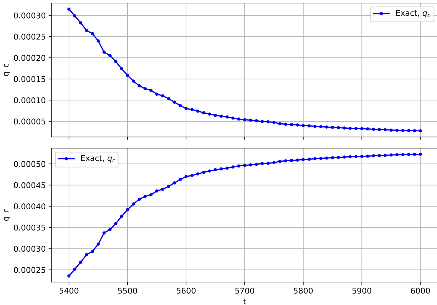
Trajectory No. 1796
