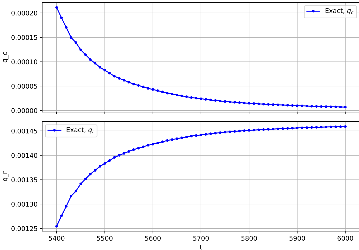
Trajectory No. 1815
