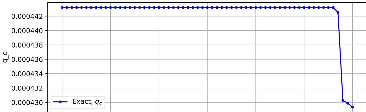
Trajectory No. 1848
