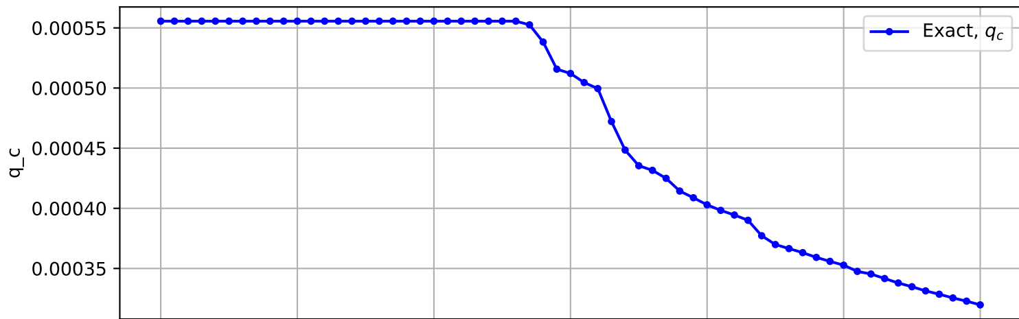
Trajectory No. 1849
