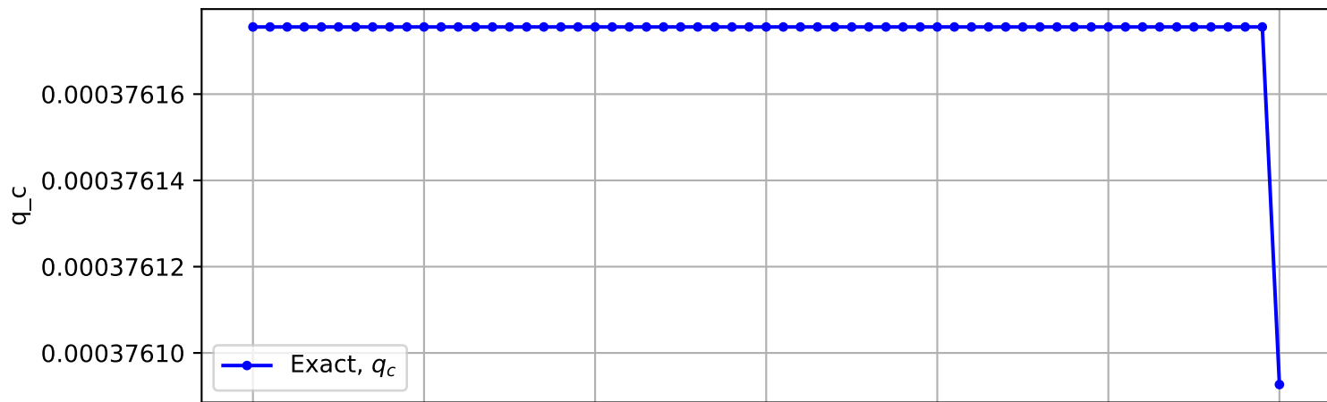
Trajectory No. 1856
