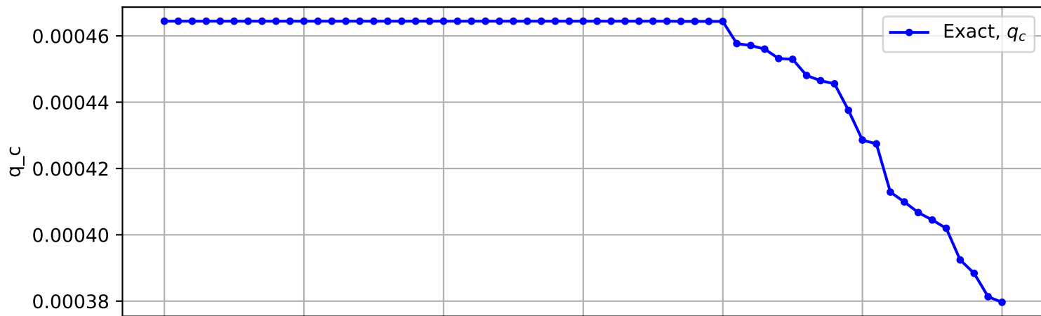
Trajectory No. 1858
