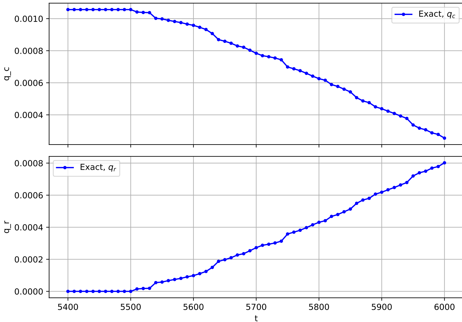
Trajectory No. 1869
