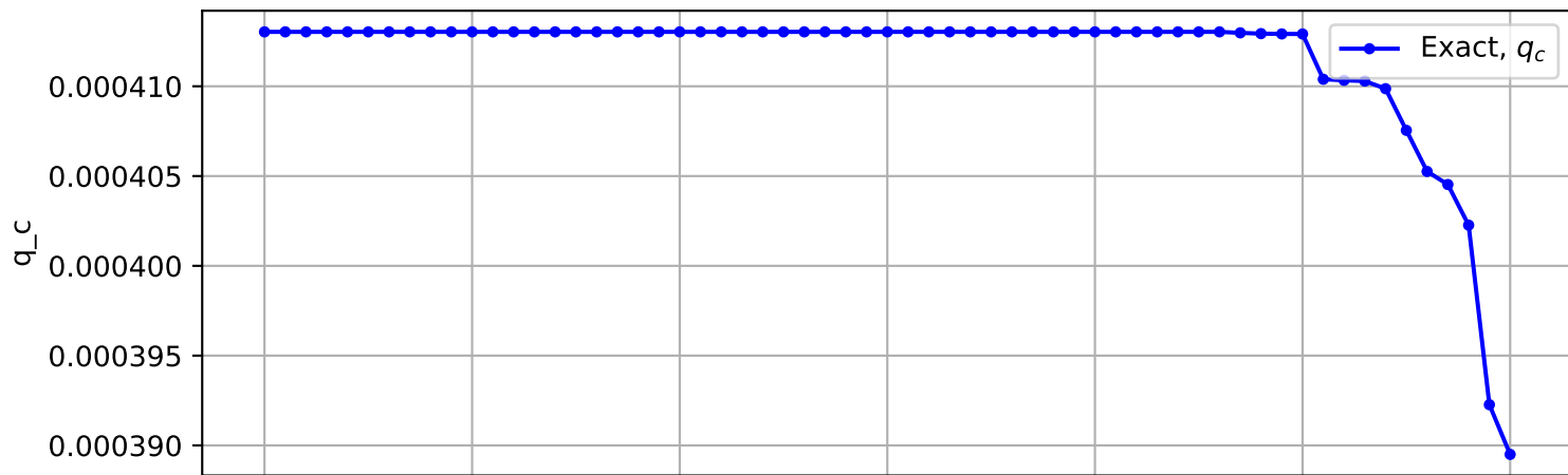
Trajectory No. 1873
