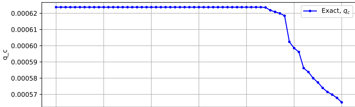
Trajectory No. 1899
