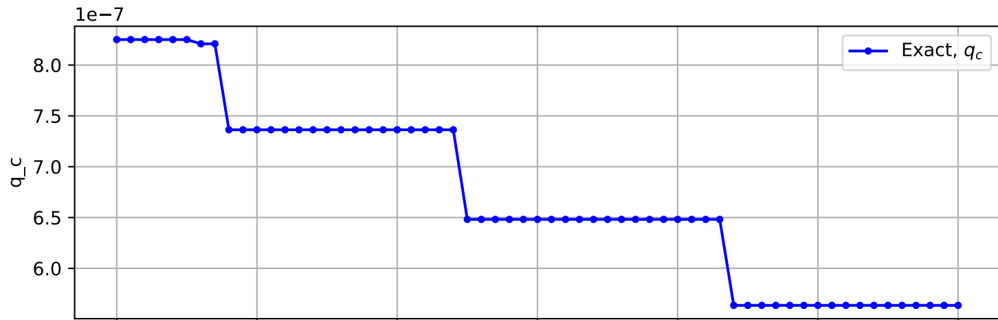
Trajectory No. 1902
