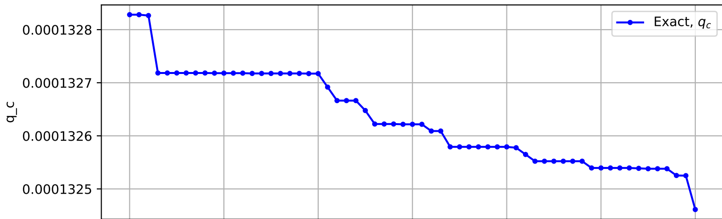
Trajectory No. 1913
