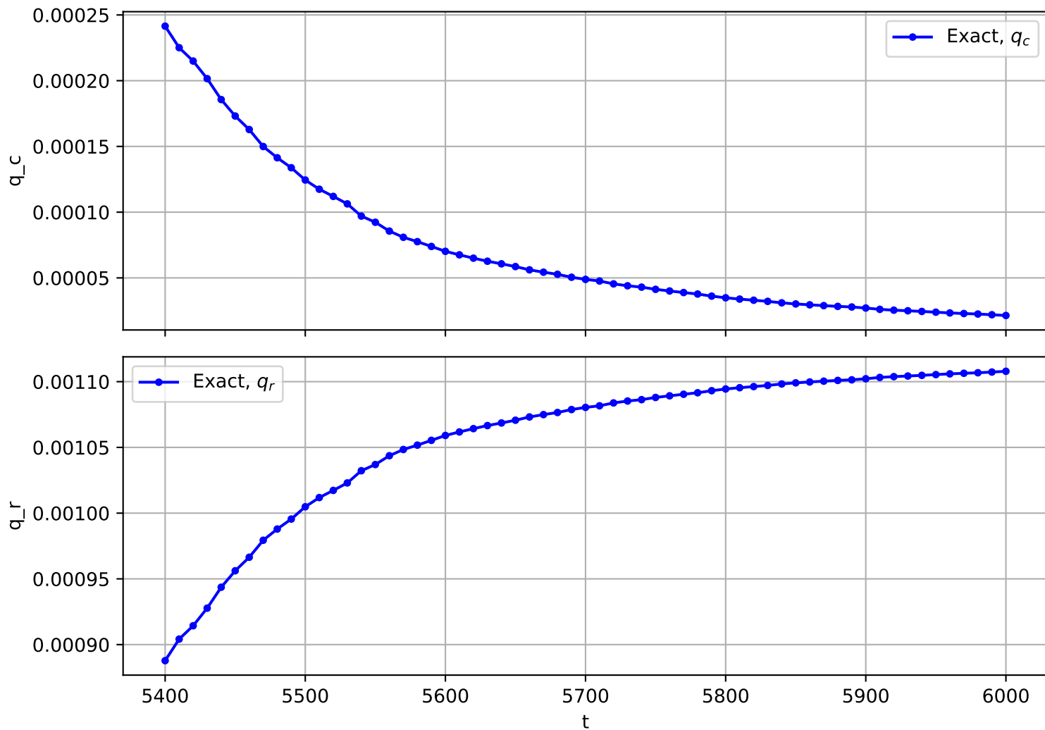
Trajectory No. 1939
