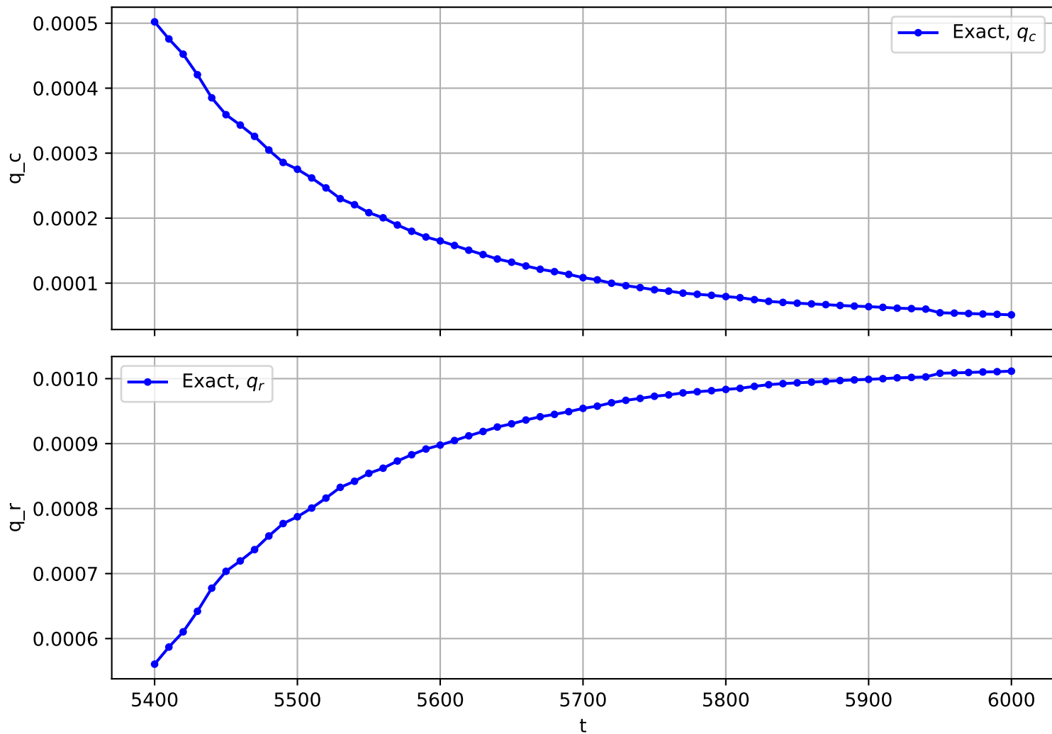
Trajectory No. 1948
