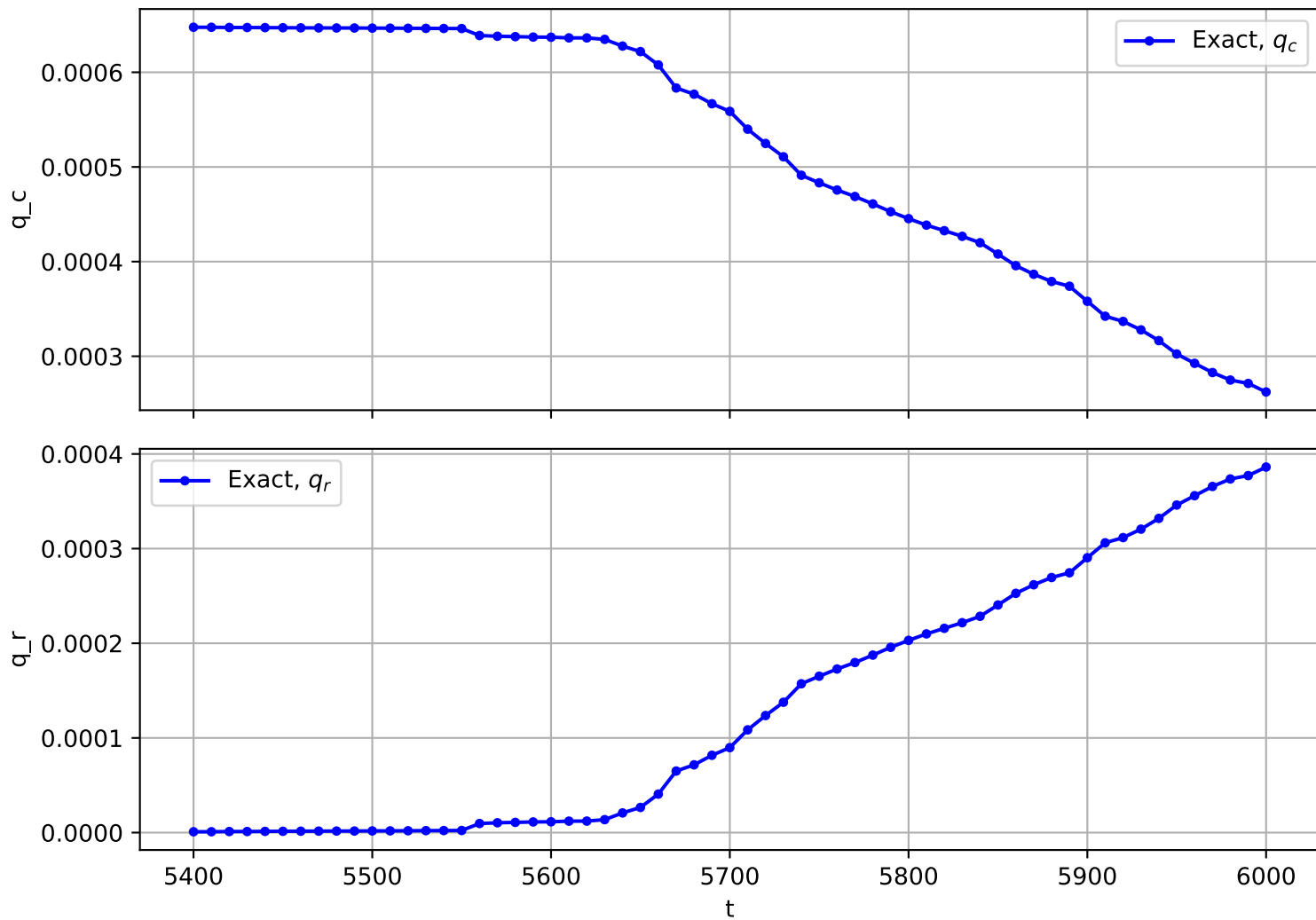
Trajectory No. 1963
