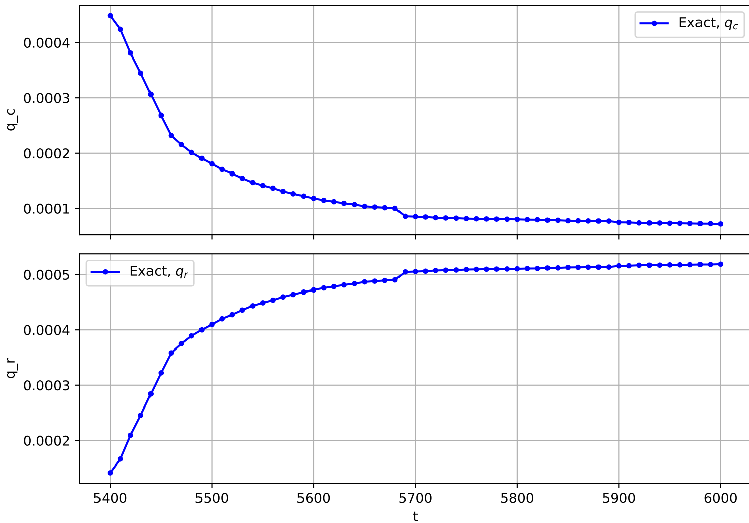
Trajectory No. 1982
