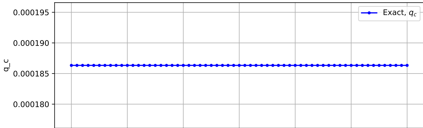
Trajectory No. 1983
