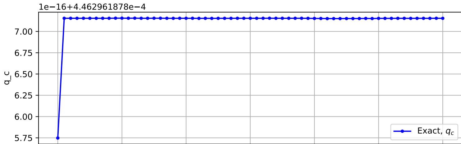
Trajectory No. 2010
