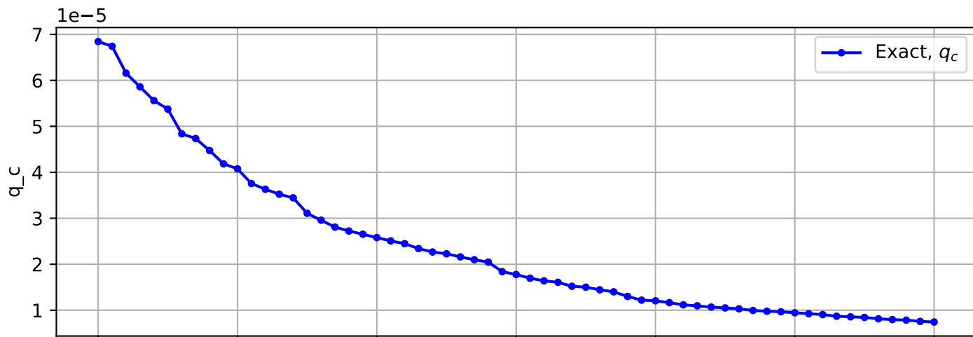
Trajectory No. 207
