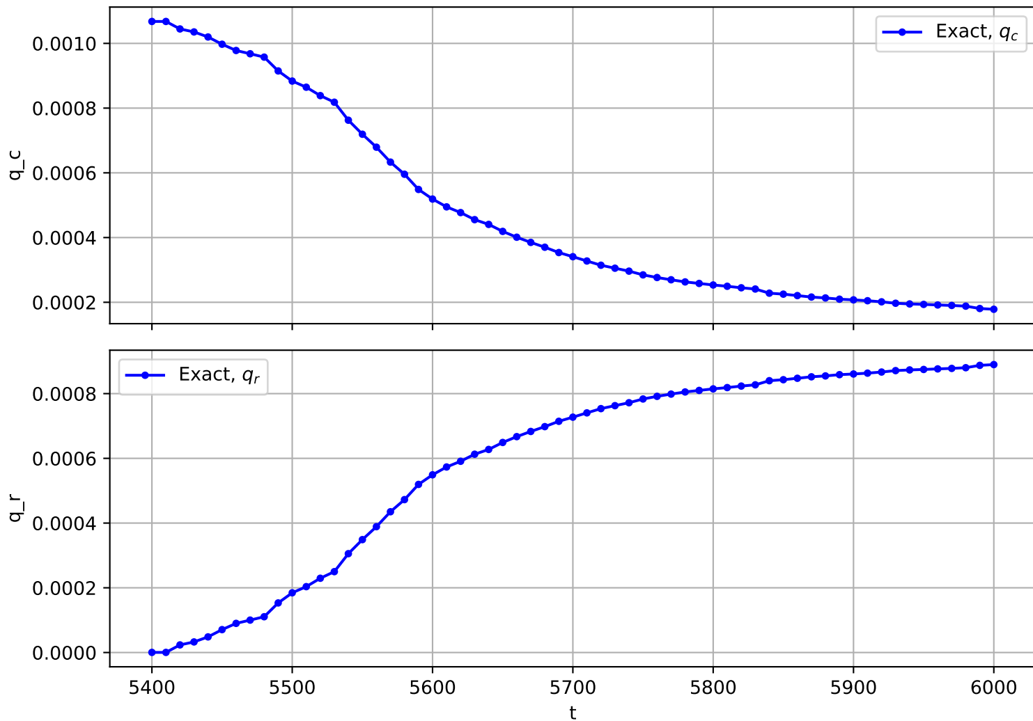
Trajectory No. 2105
