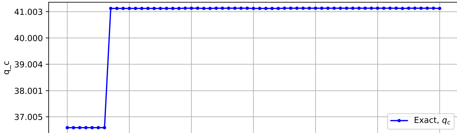
Trajectory No. 2180
