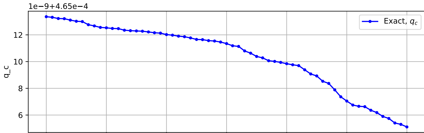
Trajectory No. 2181
