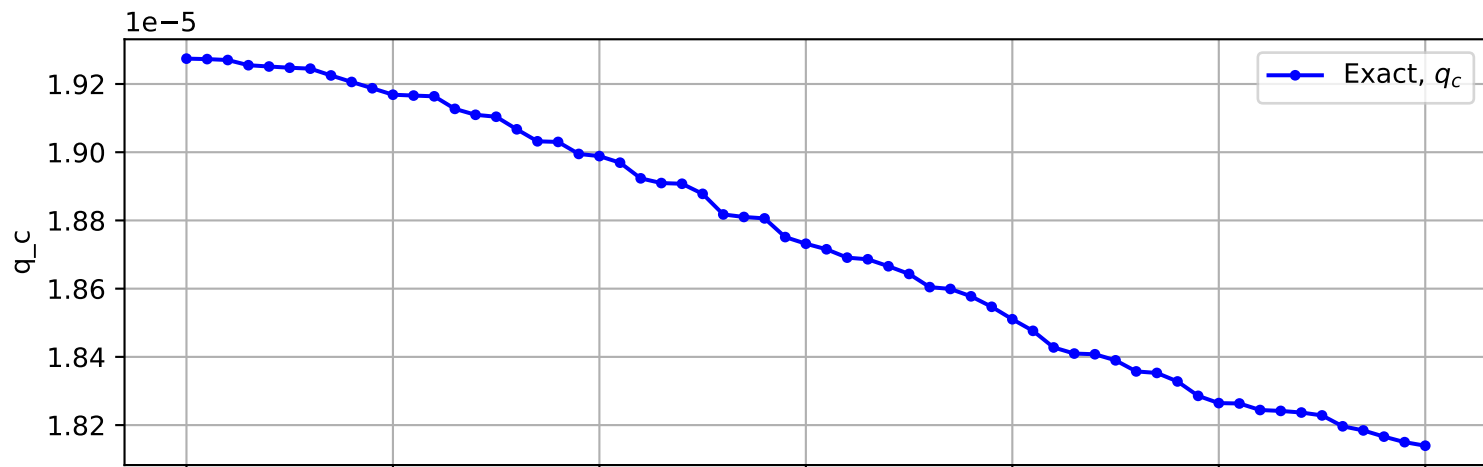
Trajectory No. 2185
