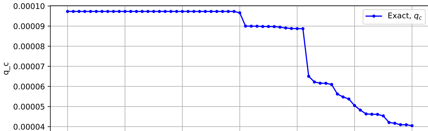
Trajectory No. 2189
