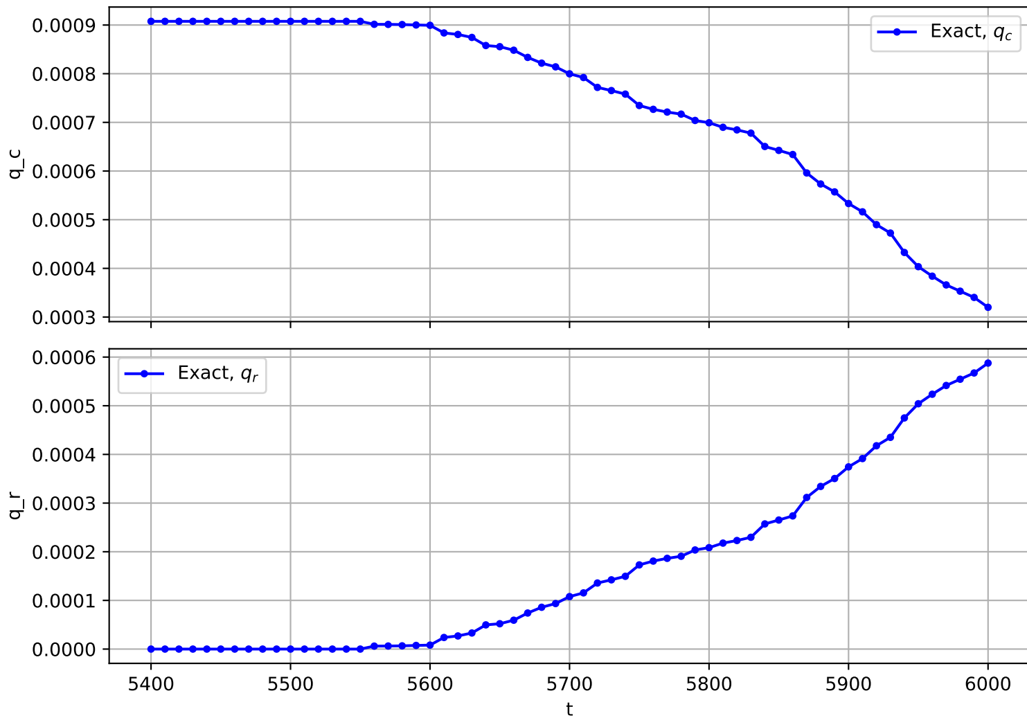
Trajectory No. 2251
