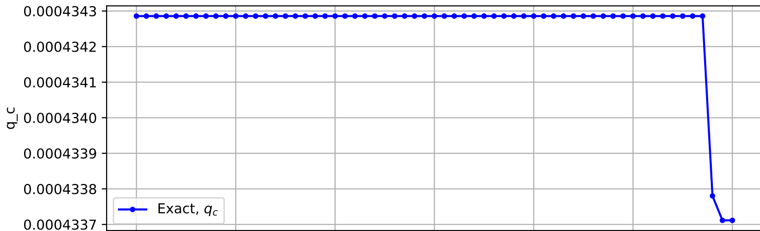
Trajectory No. 2289
