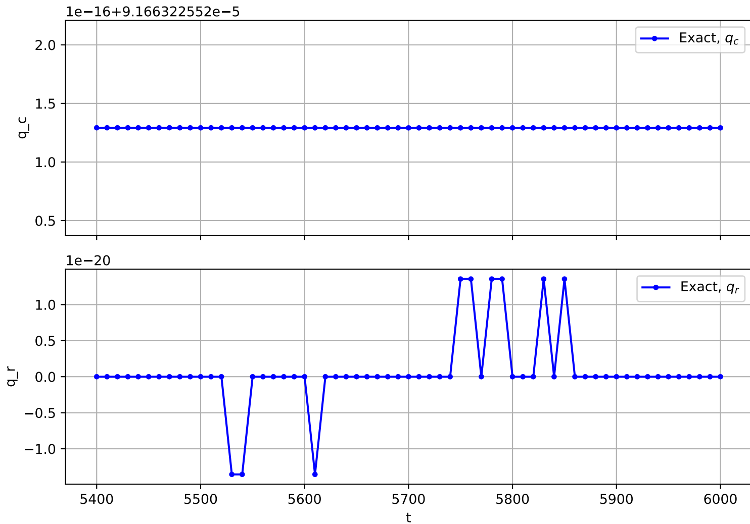
Trajectory No. 2295
