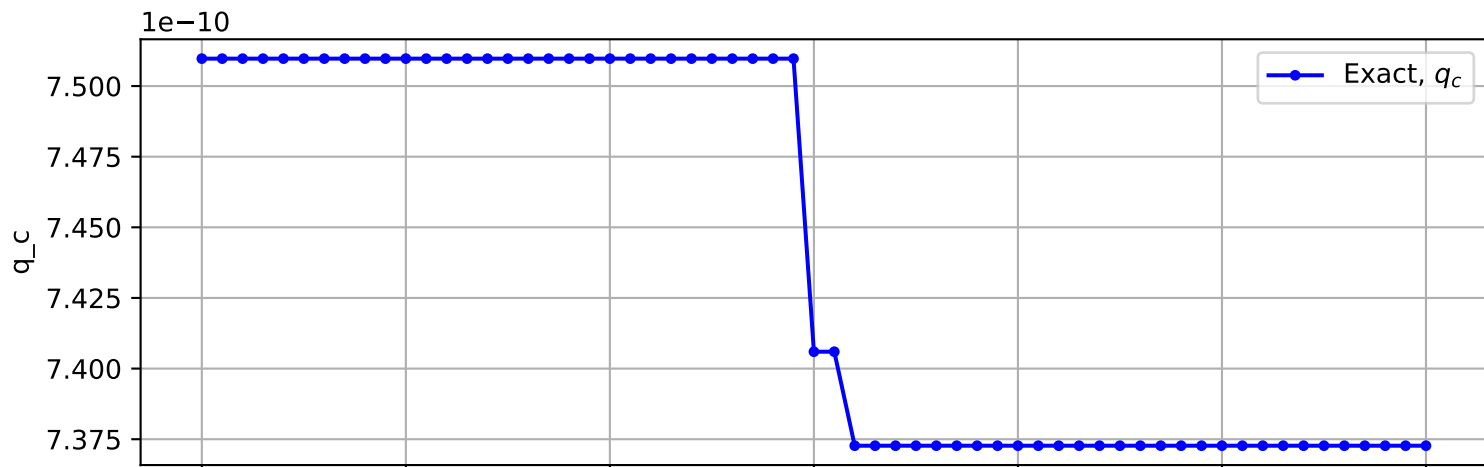
Trajectory No. 2330
