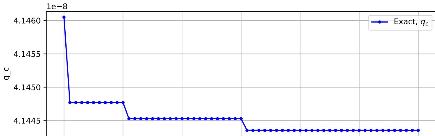
Trajectory No. 2331
