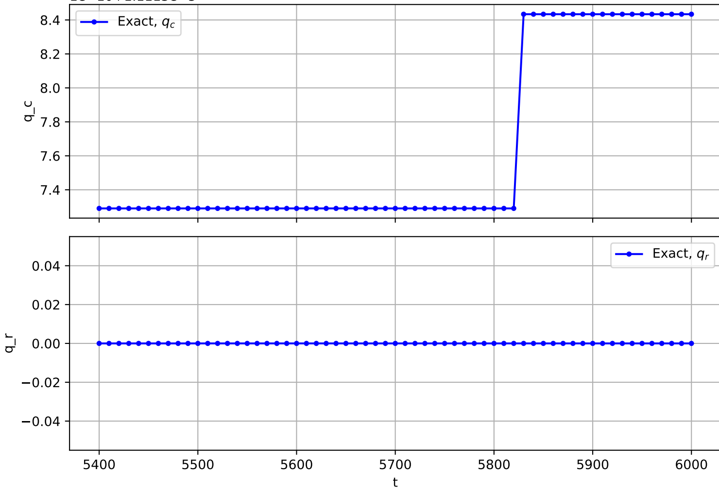
Trajectory No. 237
