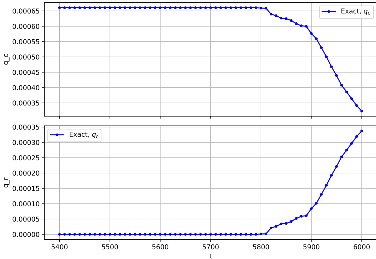
Trajectory No. 2386
